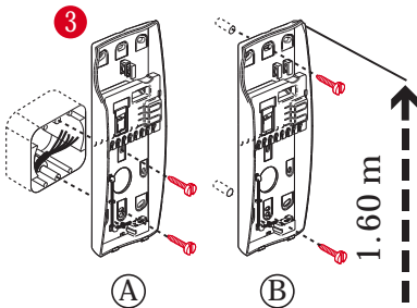
Fixing on to the universal box or wall at the recommended height
